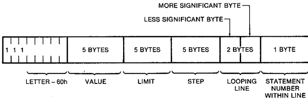
Fig. 3-9. Data structure for FOR . . . NEXT loop variable.
